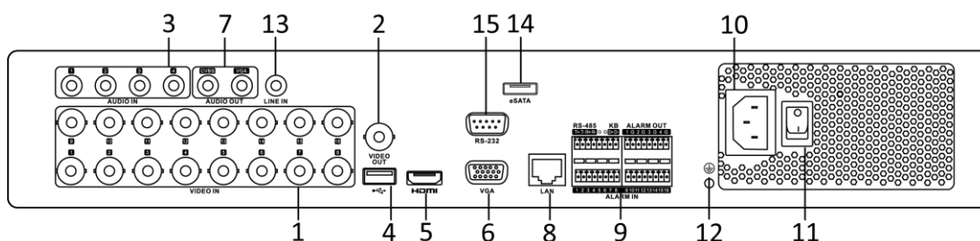
Figure 1. 13 DS-7316HQHI-SH et DS-7316HGHI-SH
