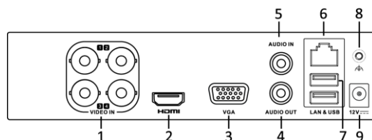
Figure 1. 10 DS-7100
