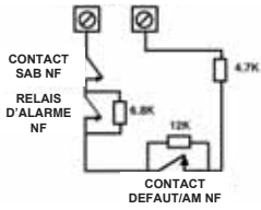
ENTREE ZONE TEOL GRADE 3
