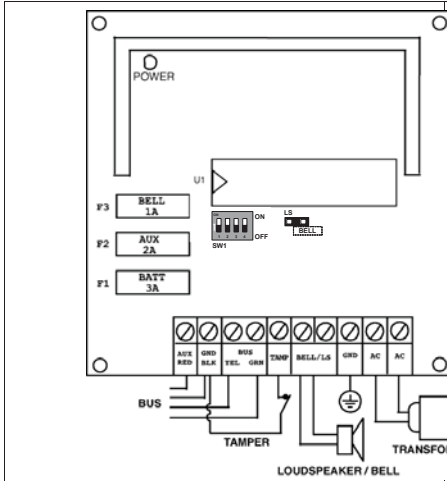
Figure 22 1.5A Power Supply Module PS
