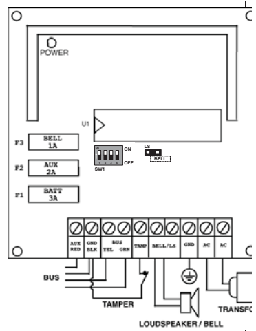
Figure 23: 3A Power Supply Module PS
